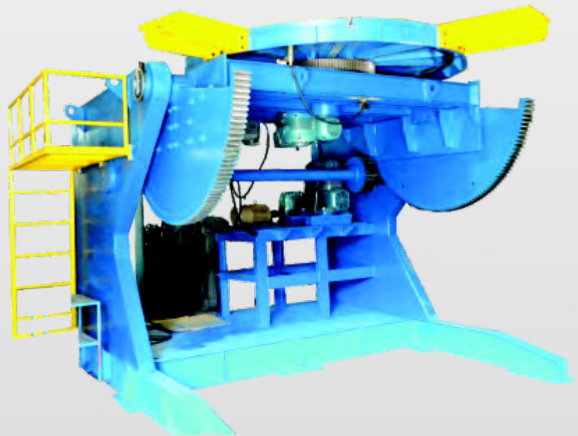
WELDING POSITIONER (15 TON)
