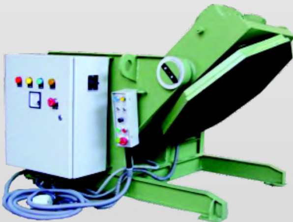
WELDING POSITIONER (5 TON)
